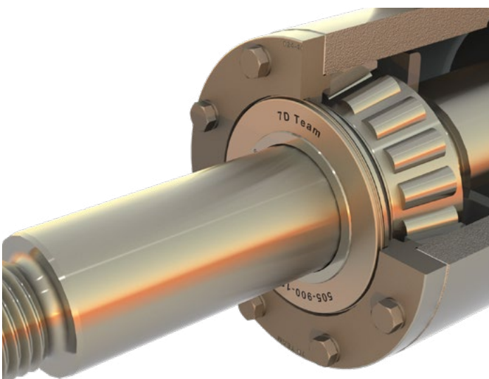
Stainless Steel Bulwark Bearing Guard in housing
